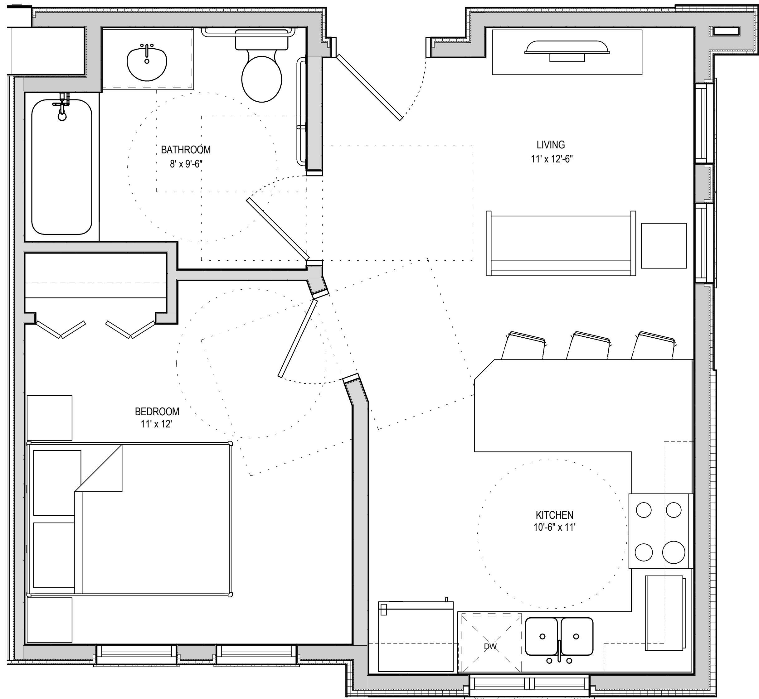
TYPE A FLOOR PLAN
